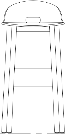
① Front View 1" = 1'-0"
