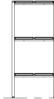
2 Side View 1/2" = 1'-0"
