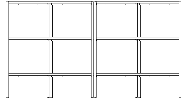
1 Front View 1/2" = 1'-0"
