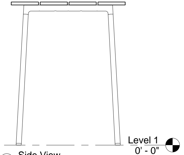
2 Side View 3/4" = 1'-0"
