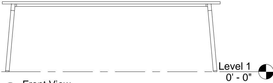
1 Front View 1/2" = 1'-0"
