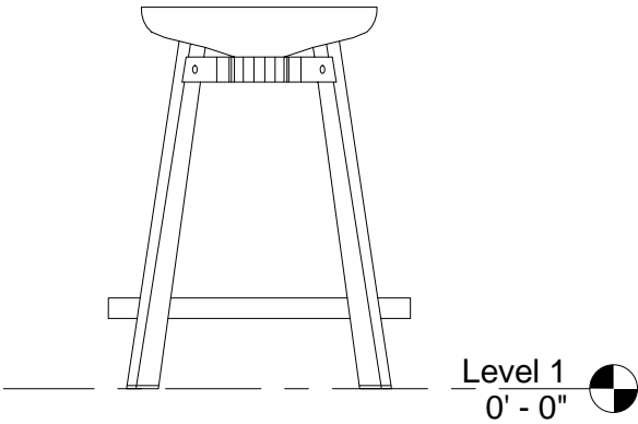
1 Front View 1" = 1'-0"
