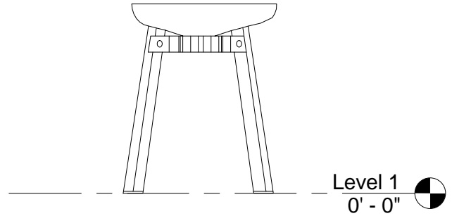
② Side View 1" = 1'-0"
